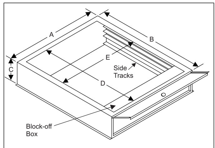
FIGURE 3 Dimensions
