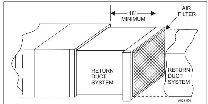
FIGURE 2 Bottom/Horizontal Mount
